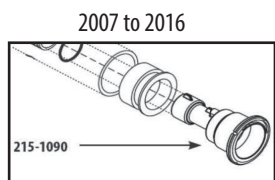
Poly Gunite Storm Spa Jet Clip-in 215-1090
