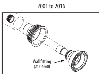
Power Gunite Storm Spa Jet Clip-in 215-6660
