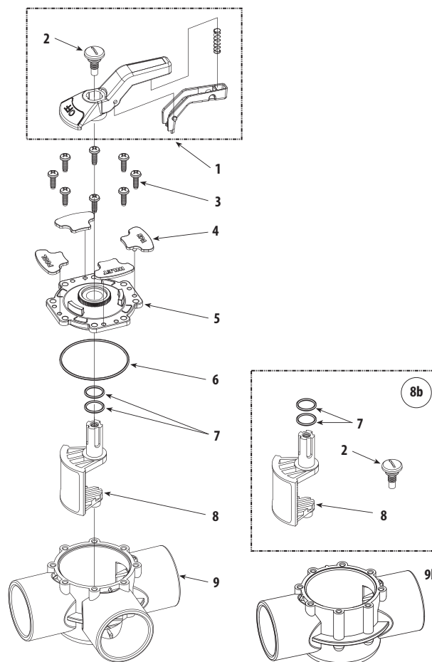
TruSeal Diverter Valve
