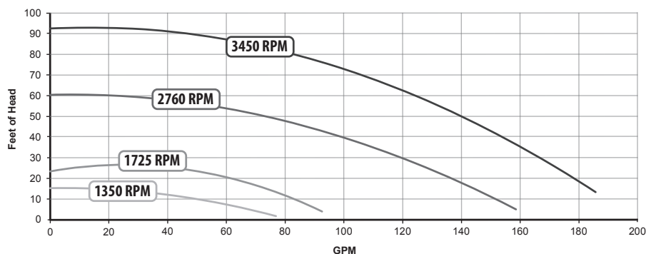
WATERWAY PD-350 Power Defender
