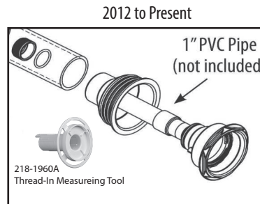
Power Gunite Storm Spa Jet Thread-In - Upgrade Kit - 400-6710 (Includes: Fitting, Threaded Ring w/ O-ring & Measuring Tool)
