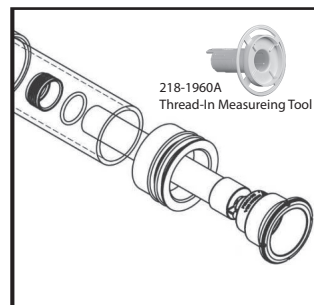
Poly Gunite Storm Spa Jet Thread-In - Upgrade Kit - 400-1190 (Includes: Fitting, Threaded Ring w/ O-ring & Measuring Tool)
