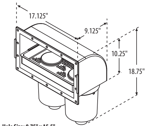
Hole Size: 8.75" x 15.5"
